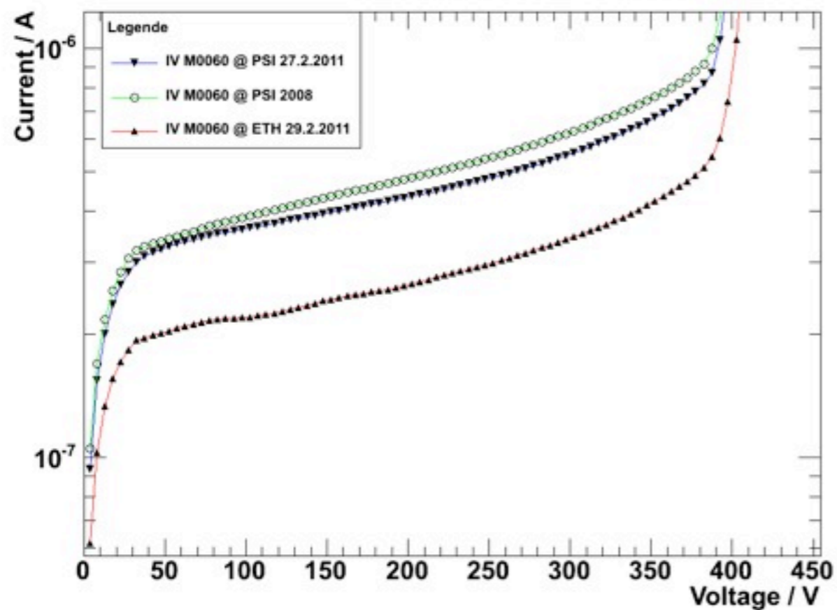
IV-Curves of M0060 @ ETH and PSI
