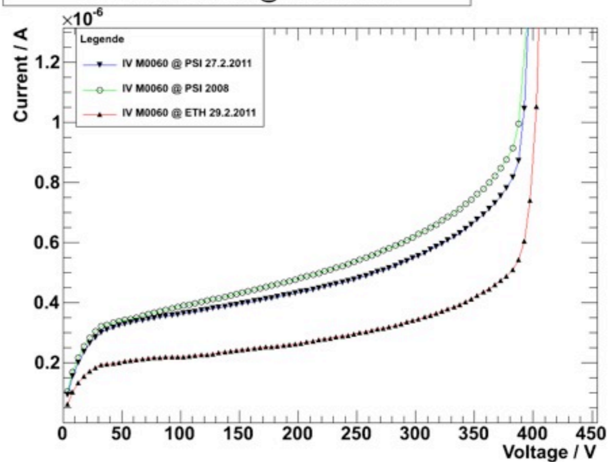
IV-Curves of M0060 @ ETH and PSI
