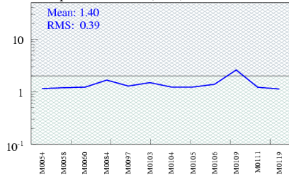
IVslope at T = -10^{\circ}\text{C} (ATC)
