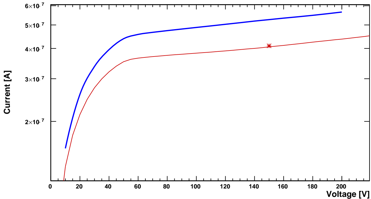
I-V-Curve
