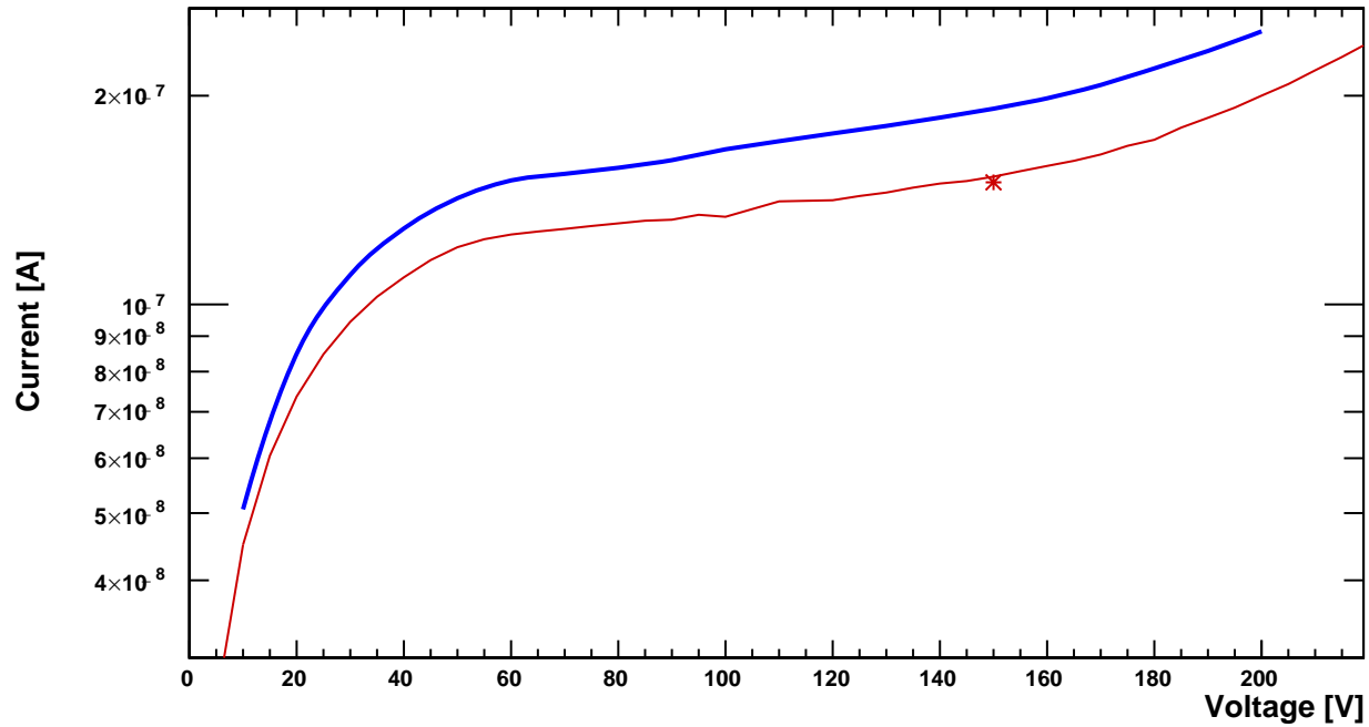
I-V-Curve
