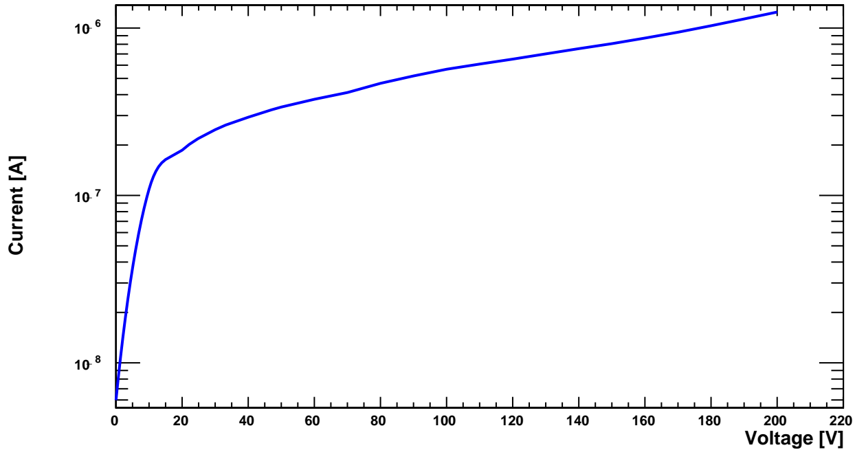
I-V-Curve
