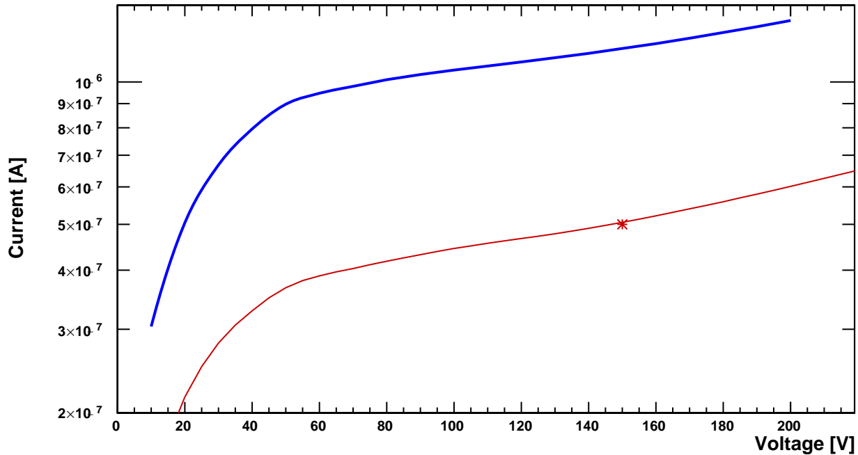
I-V-Curve
