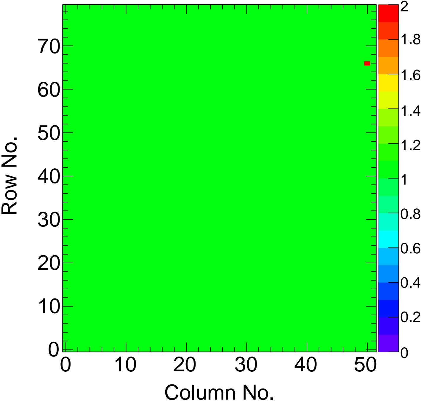
Bare BBMap: C6
