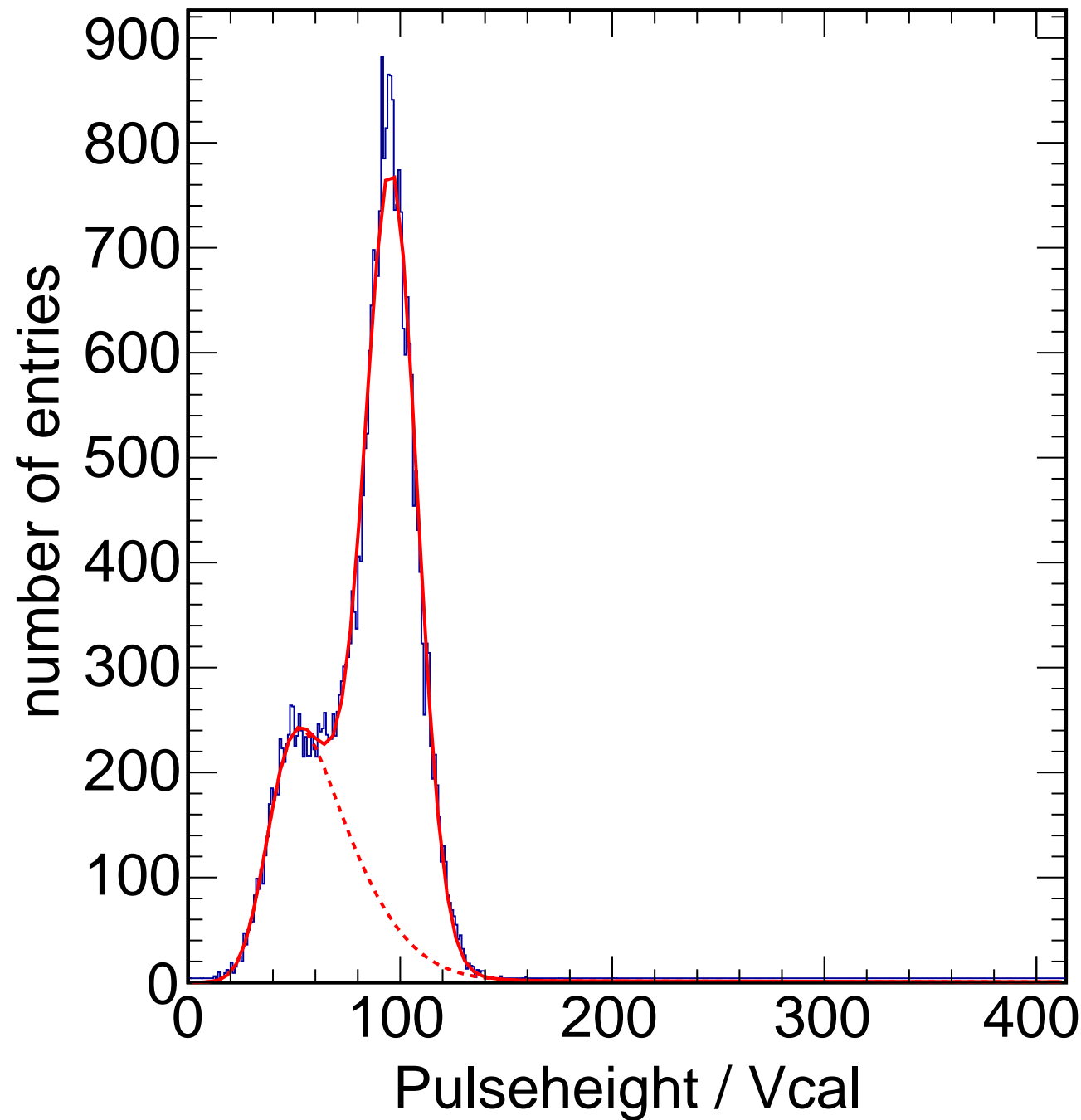
X-ray Calibration - Target Mo Method Spectrum Chip C15
