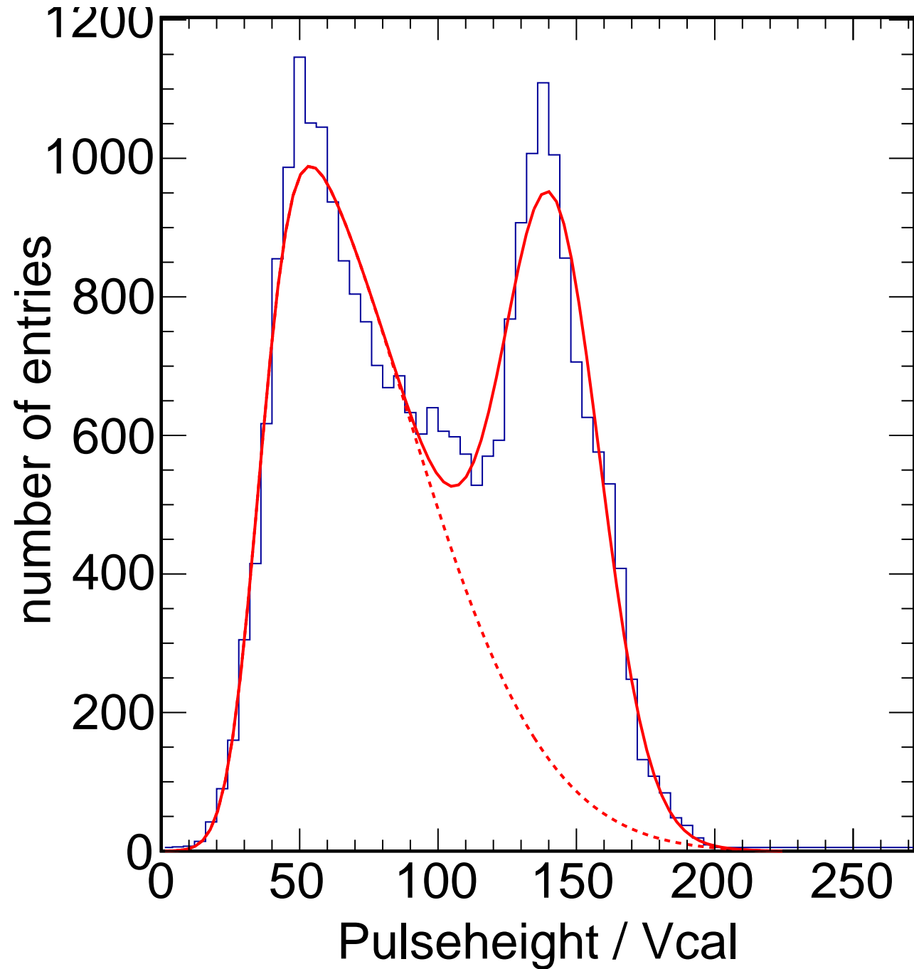
X-ray Calibration - Target Sn Method Spectrum Chip C10
