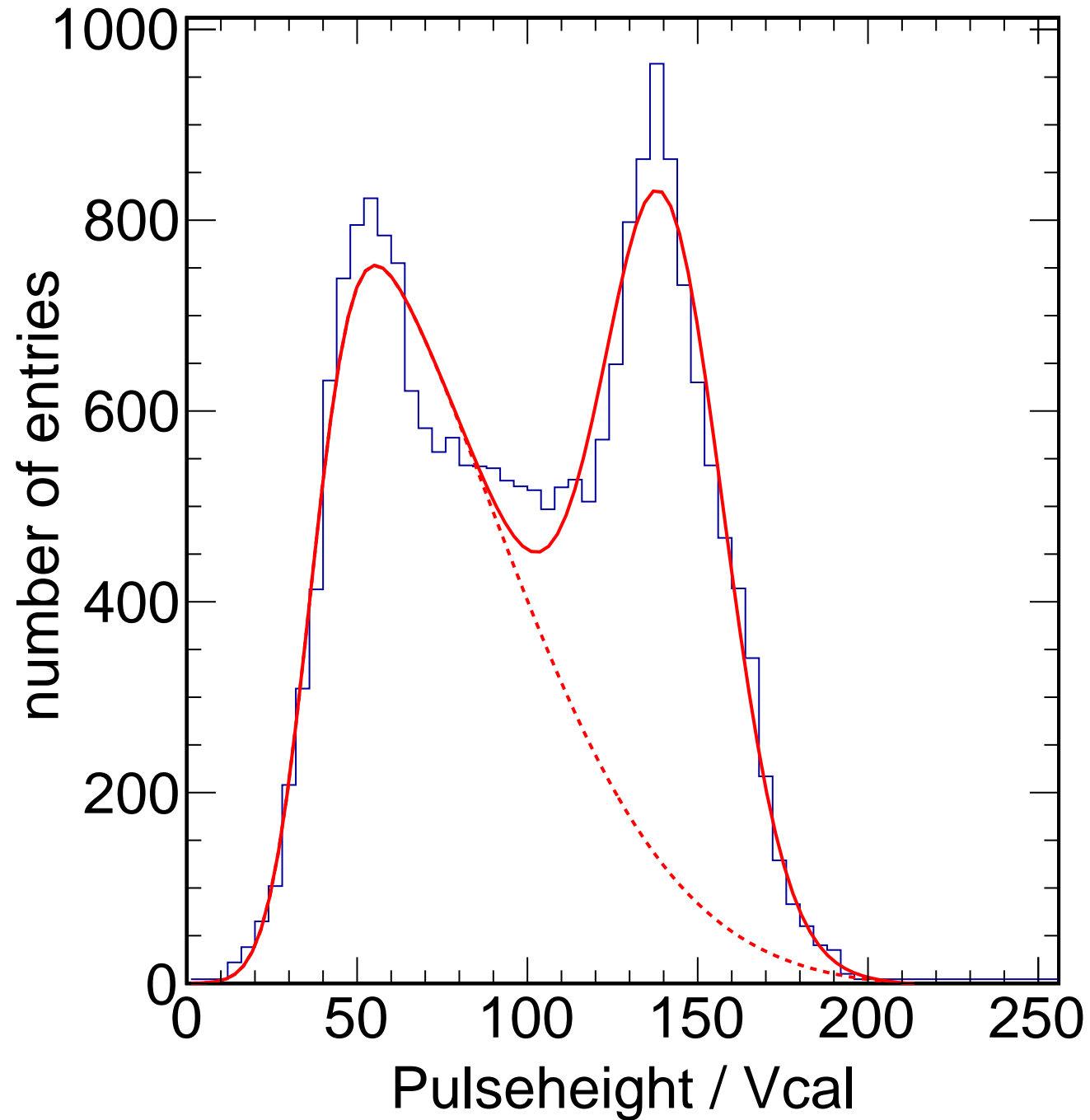
X-ray Calibration - Target Sn Method Spectrum Chip C14
