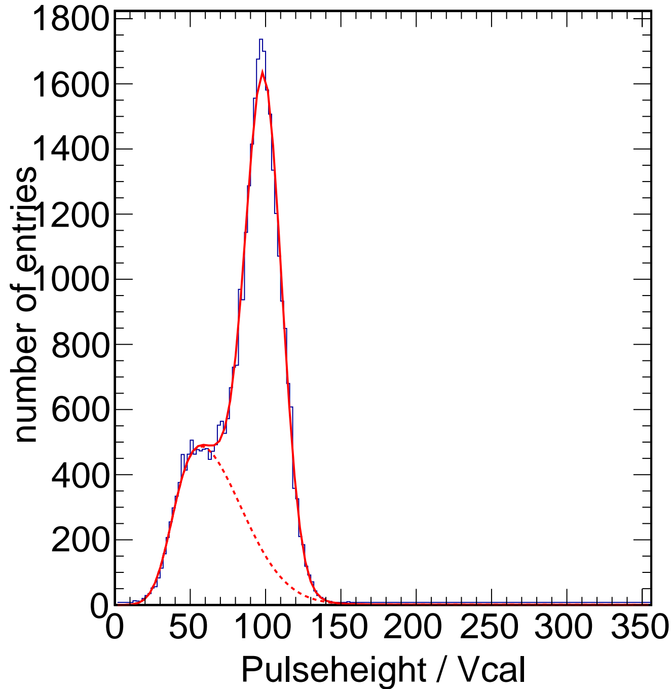
X-ray Calibration - Target Mo Method Spectrum Chip C6
