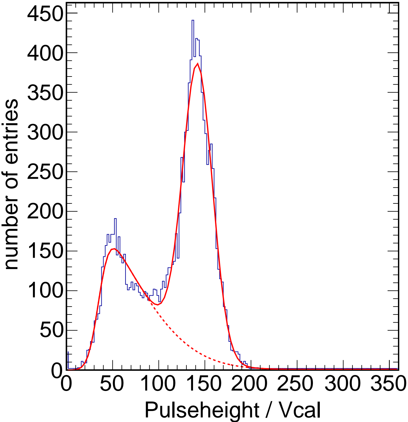
X-ray Calibration - Target Sn Method Spectrum Chip C1
