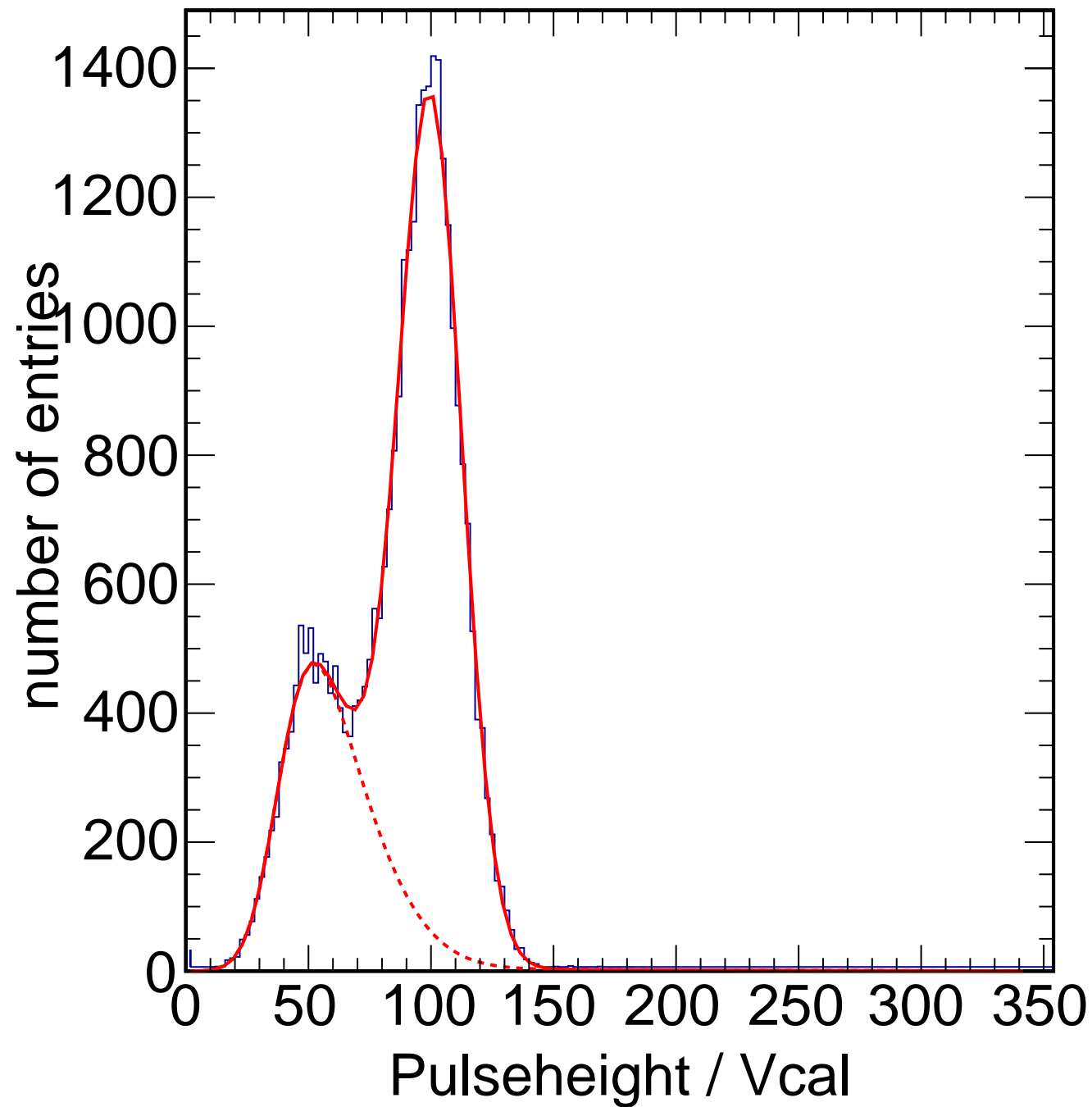
X-ray Calibration - Target Mo Method Spectrum Chip C1
