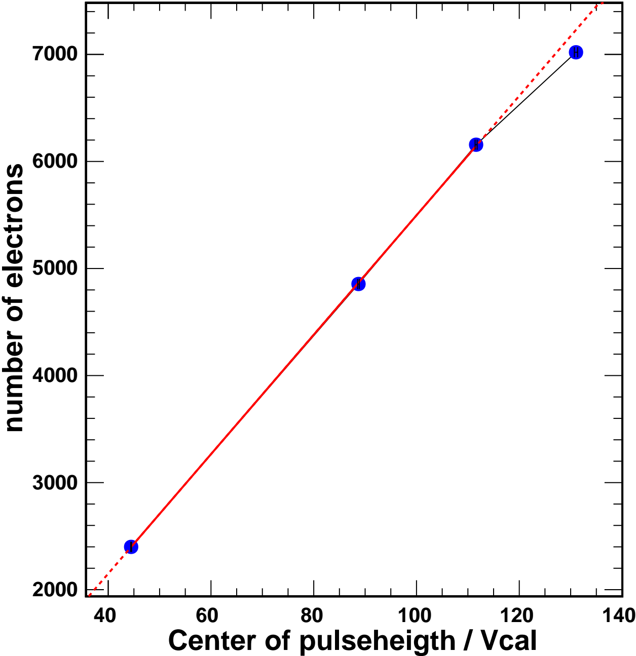
X-ray Calibration - Vcal Calibration Method Spectrum Chip C9
