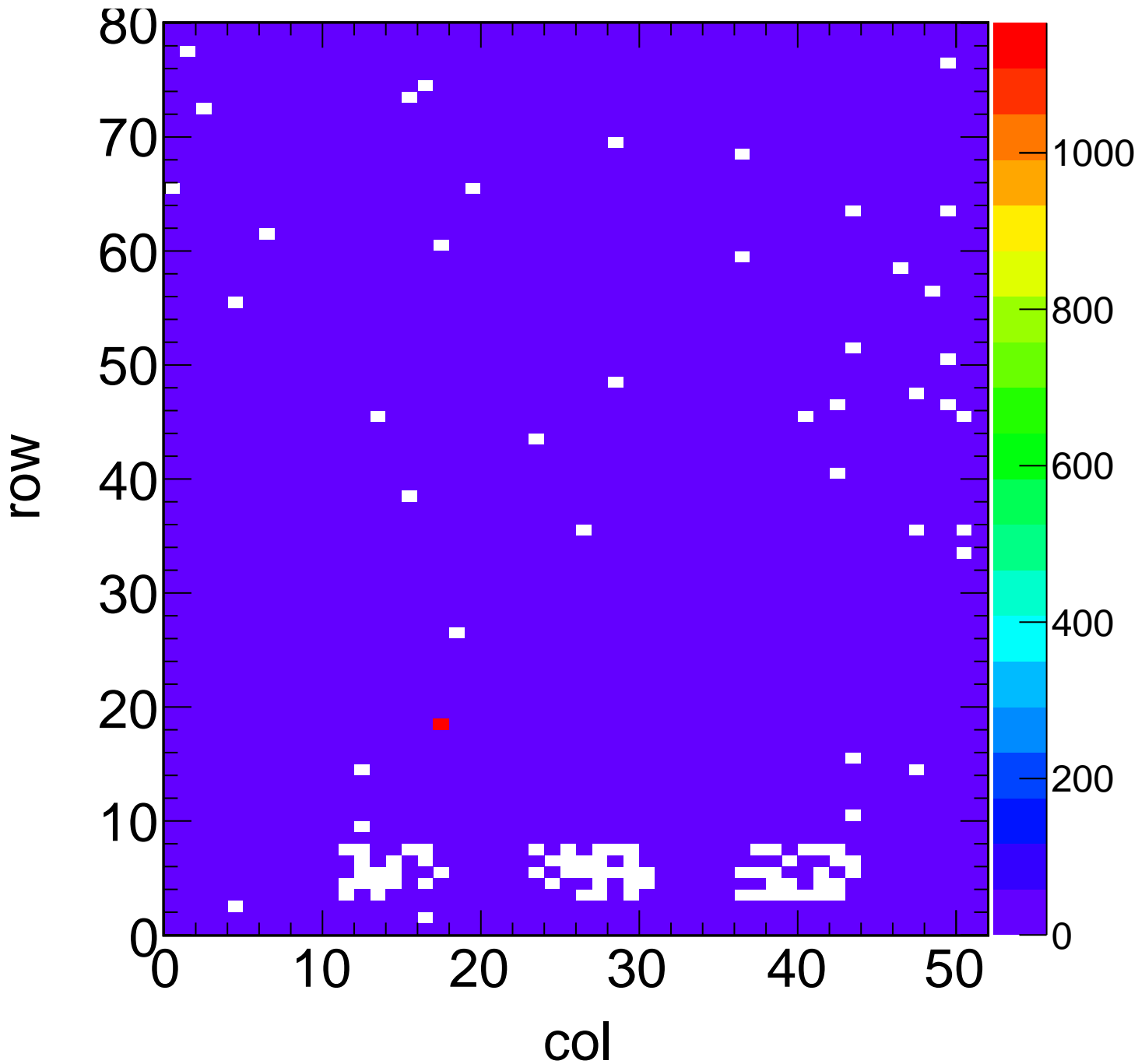
X-ray Hit Map - Target Sn Method Spectrum Chip C1
