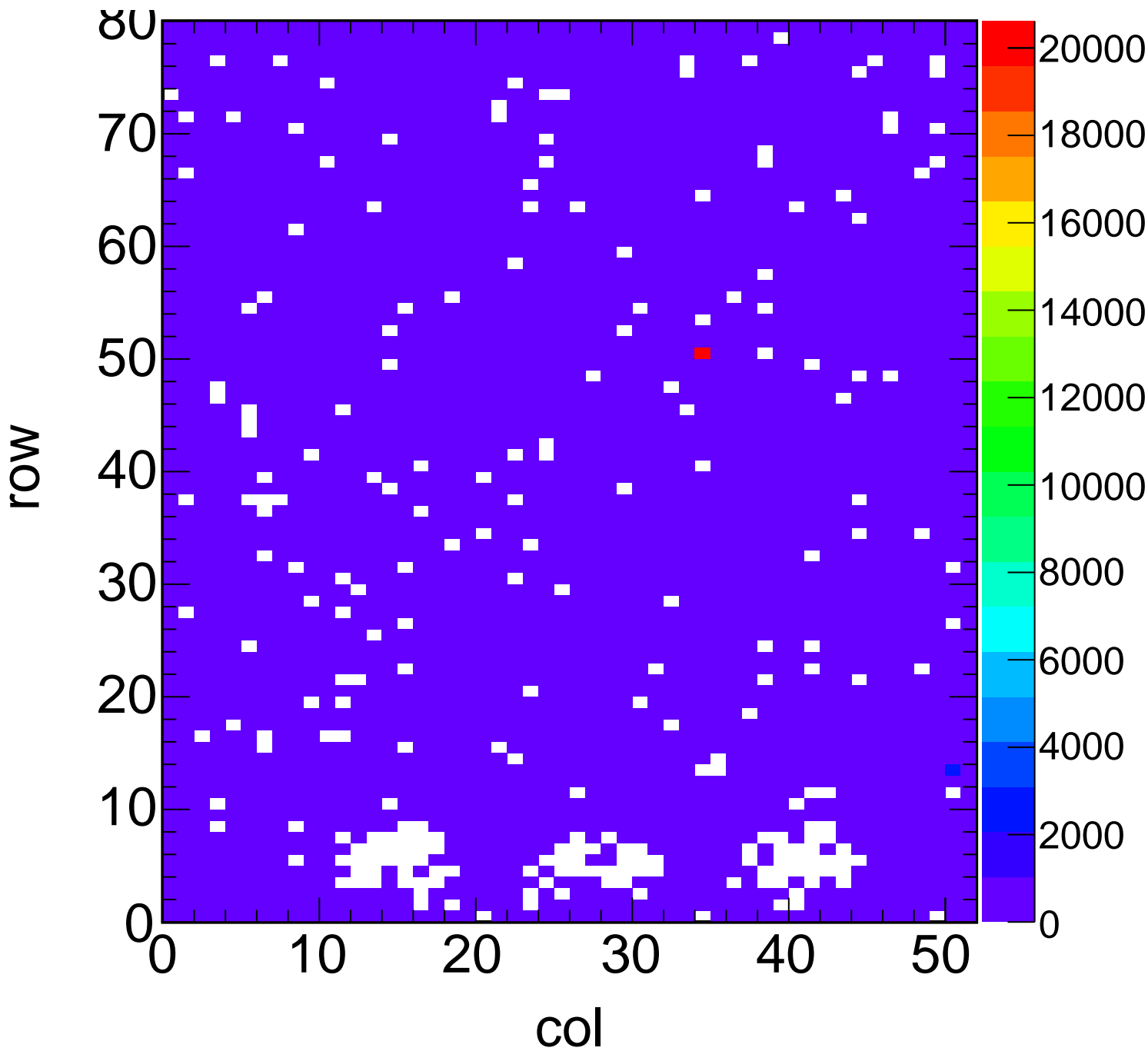
X-ray Hit Map - Target Sn Method Spectrum Chip C10
