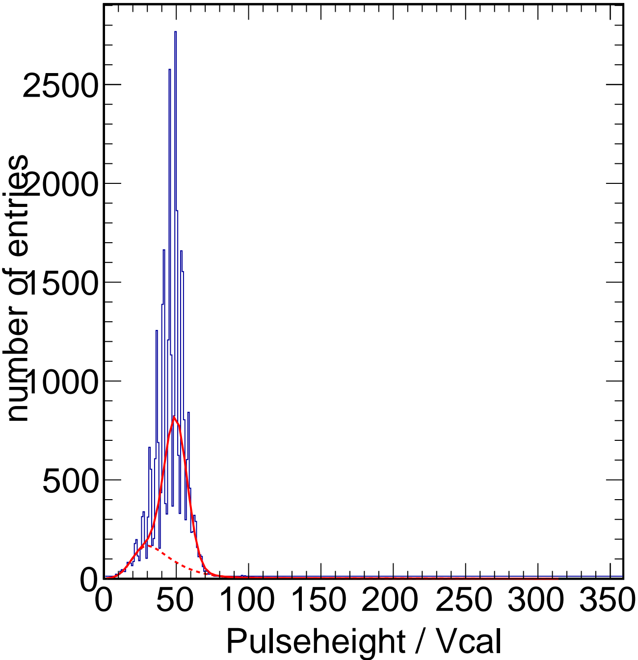
X-ray Calibration - Target Zn Method Spectrum Chip C5
