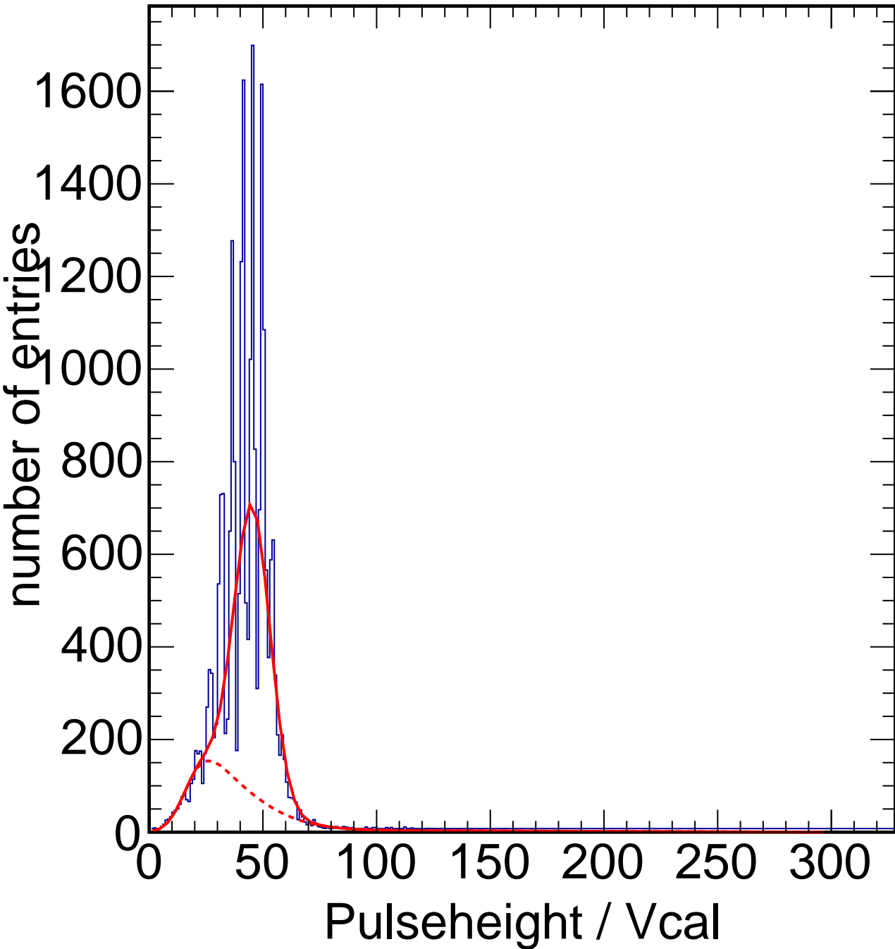
X-ray Calibration - Target Zn Method Spectrum Chip C8
