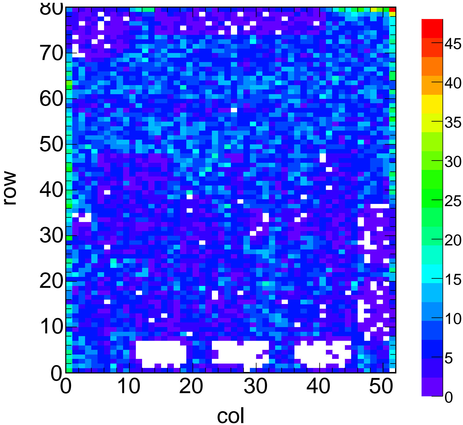
X-ray Hit Map - Target Zn Method Spectrum Chip C7
