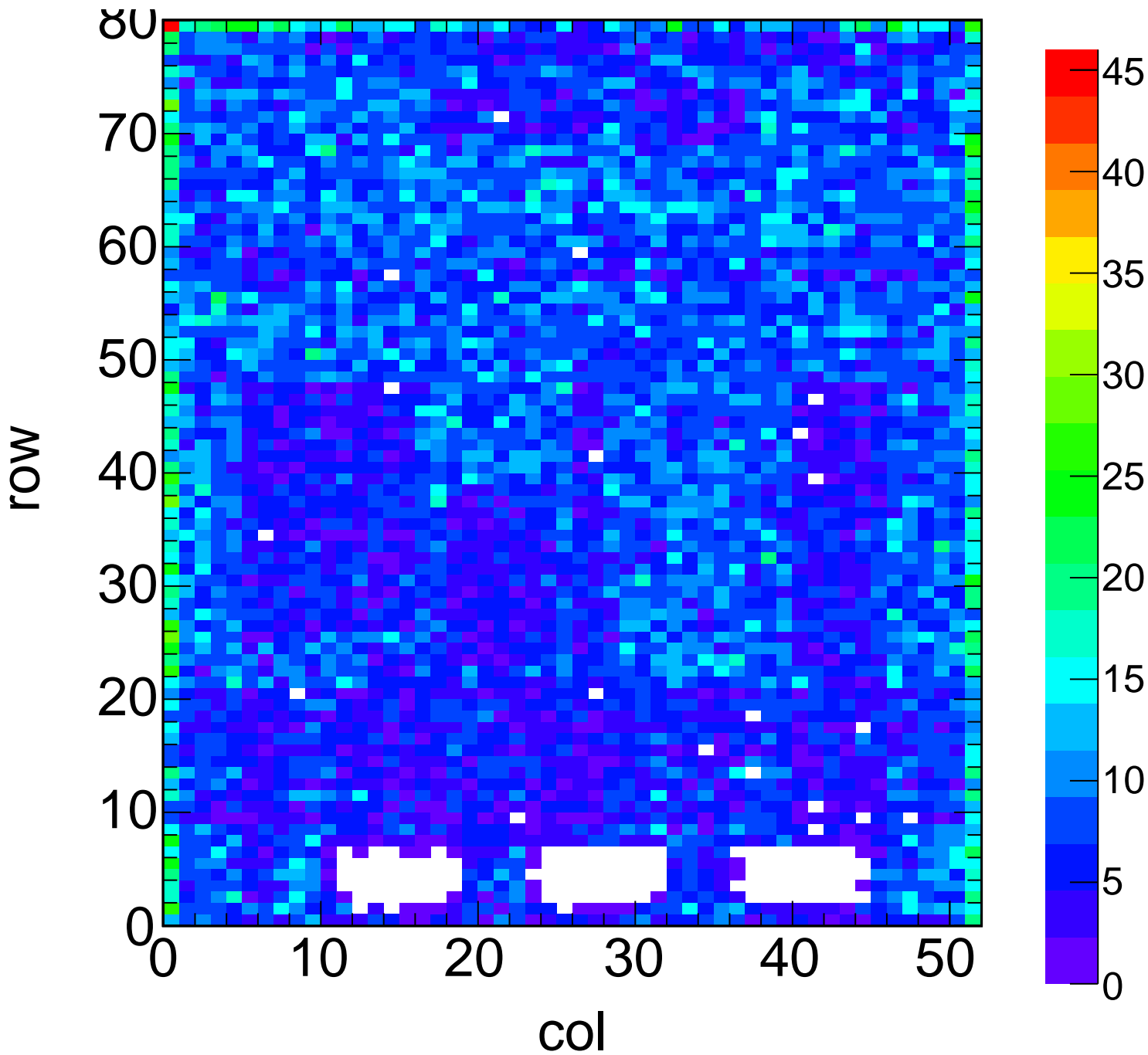
X-ray Hit Map - Target Zn Method Spectrum Chip C5
