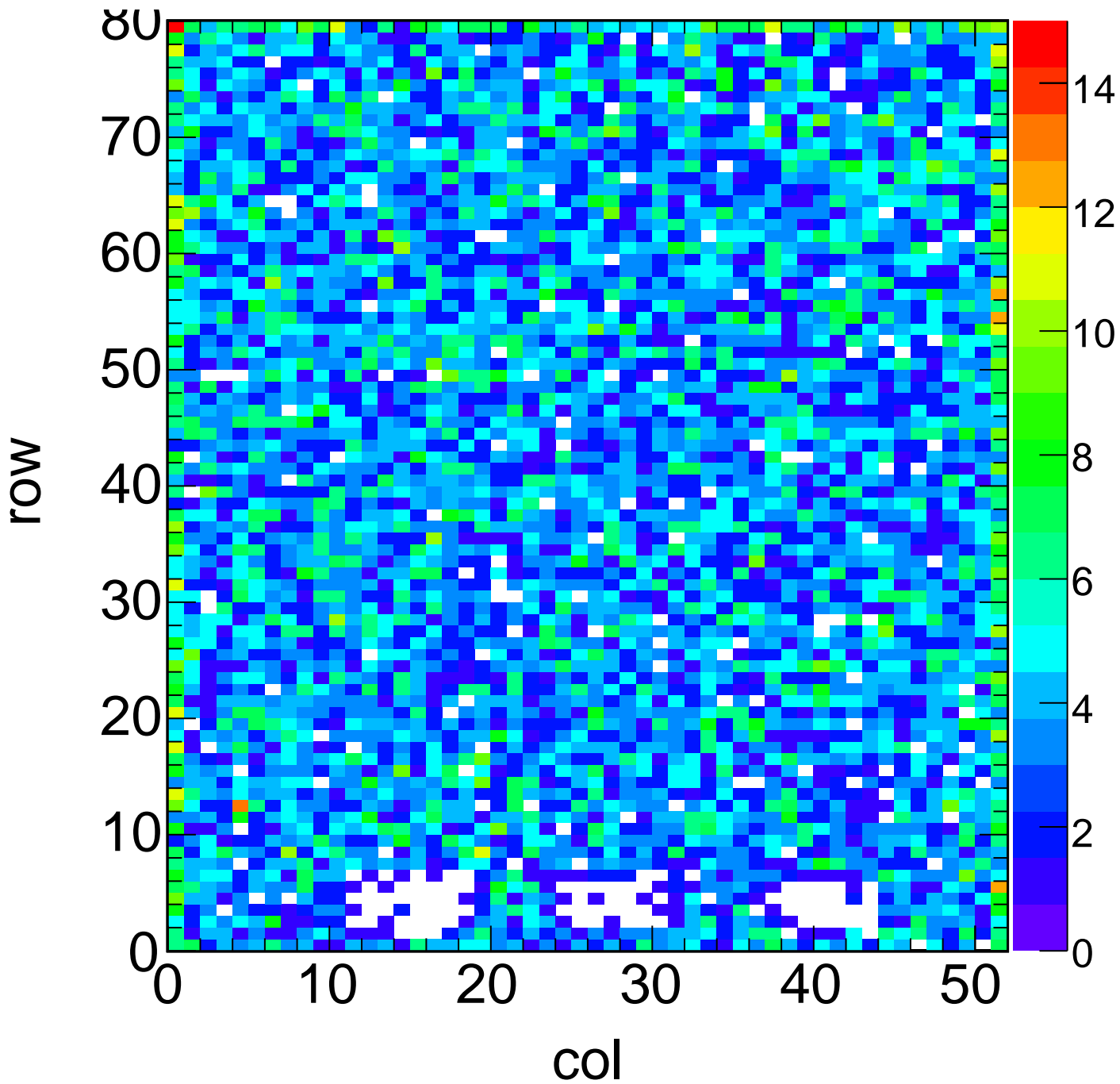
X-ray Hit Map - Target Sn Method Spectrum Chip C5
