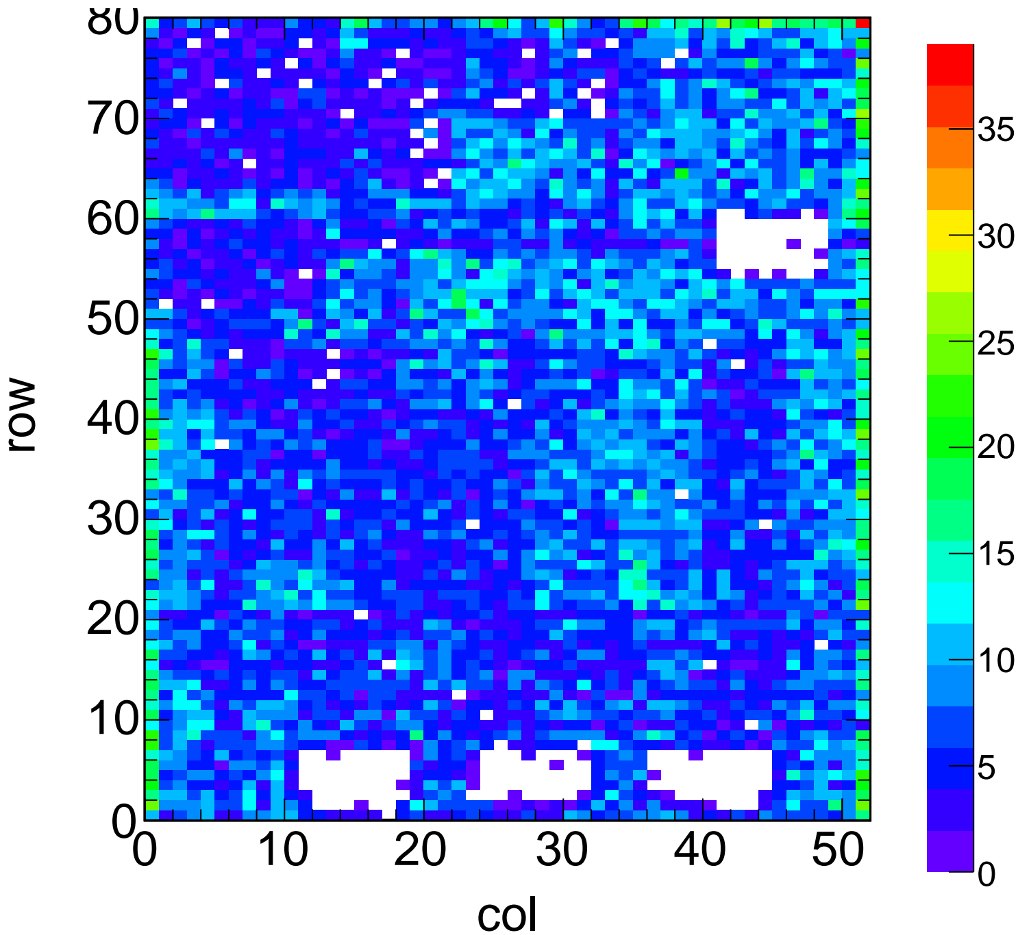
X-ray Hit Map - Target Zn Method Spectrum Chip C4
