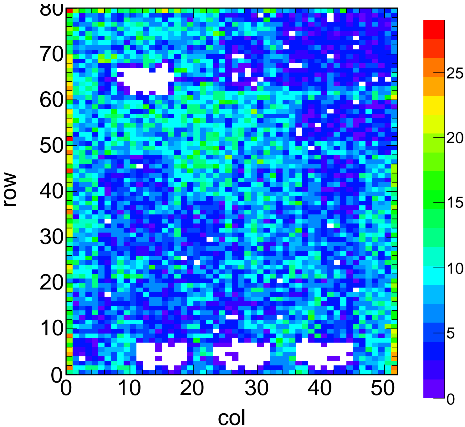
X-ray Hit Map - Target Zn Method Spectrum Chip C3
