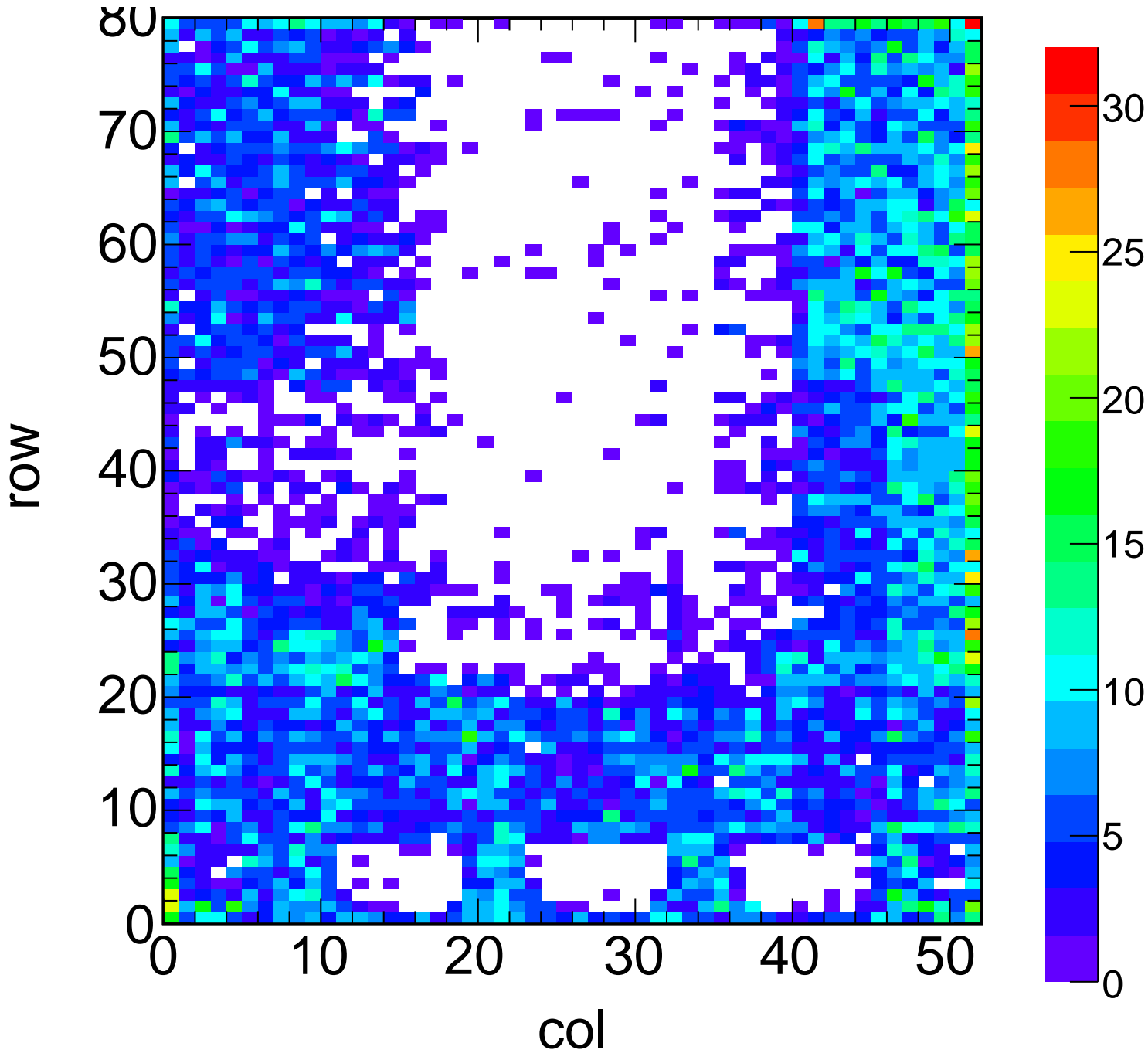
X-ray Hit Map - Target Zn Method Spectrum Chip C2
