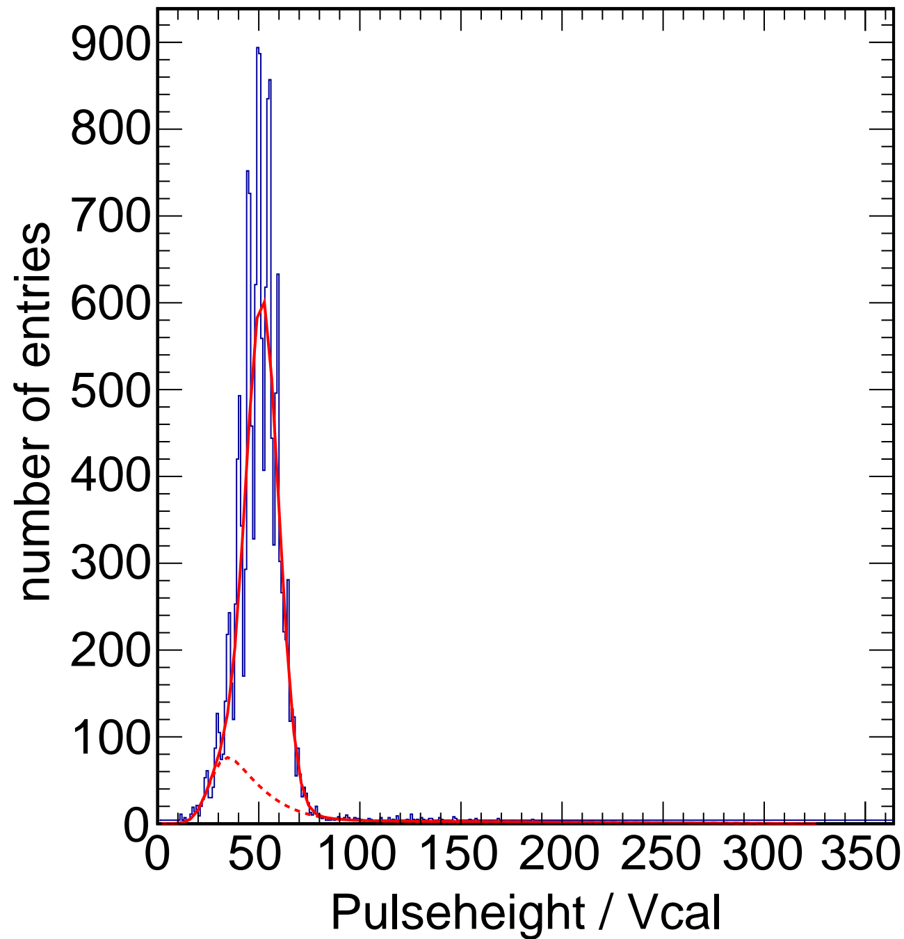
X-ray Calibration - Target Zn Method Spectrum Chip C13
