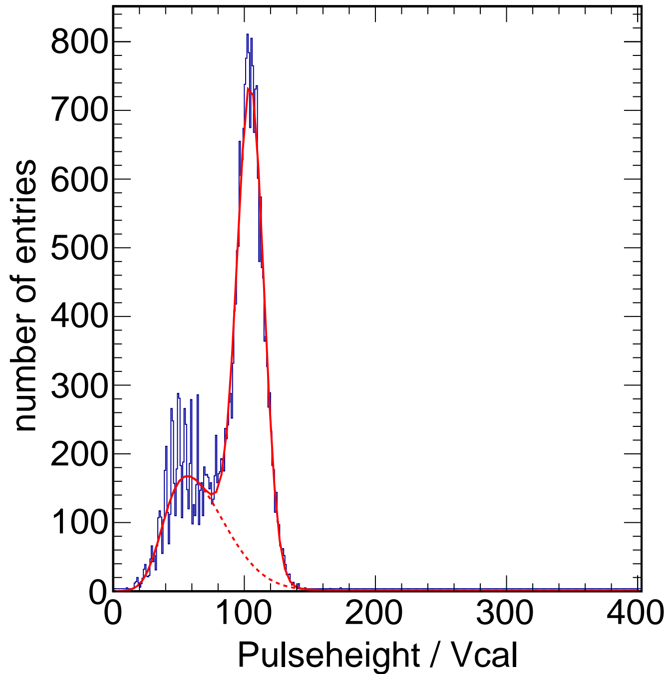
X-ray Calibration - Target Mo Method Spectrum Chip C13
