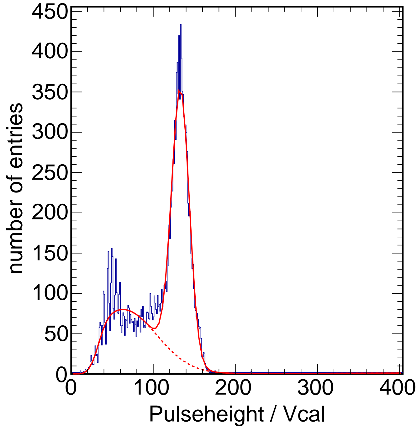
X-ray Calibration - Target Ag Method Spectrum Chip C13
