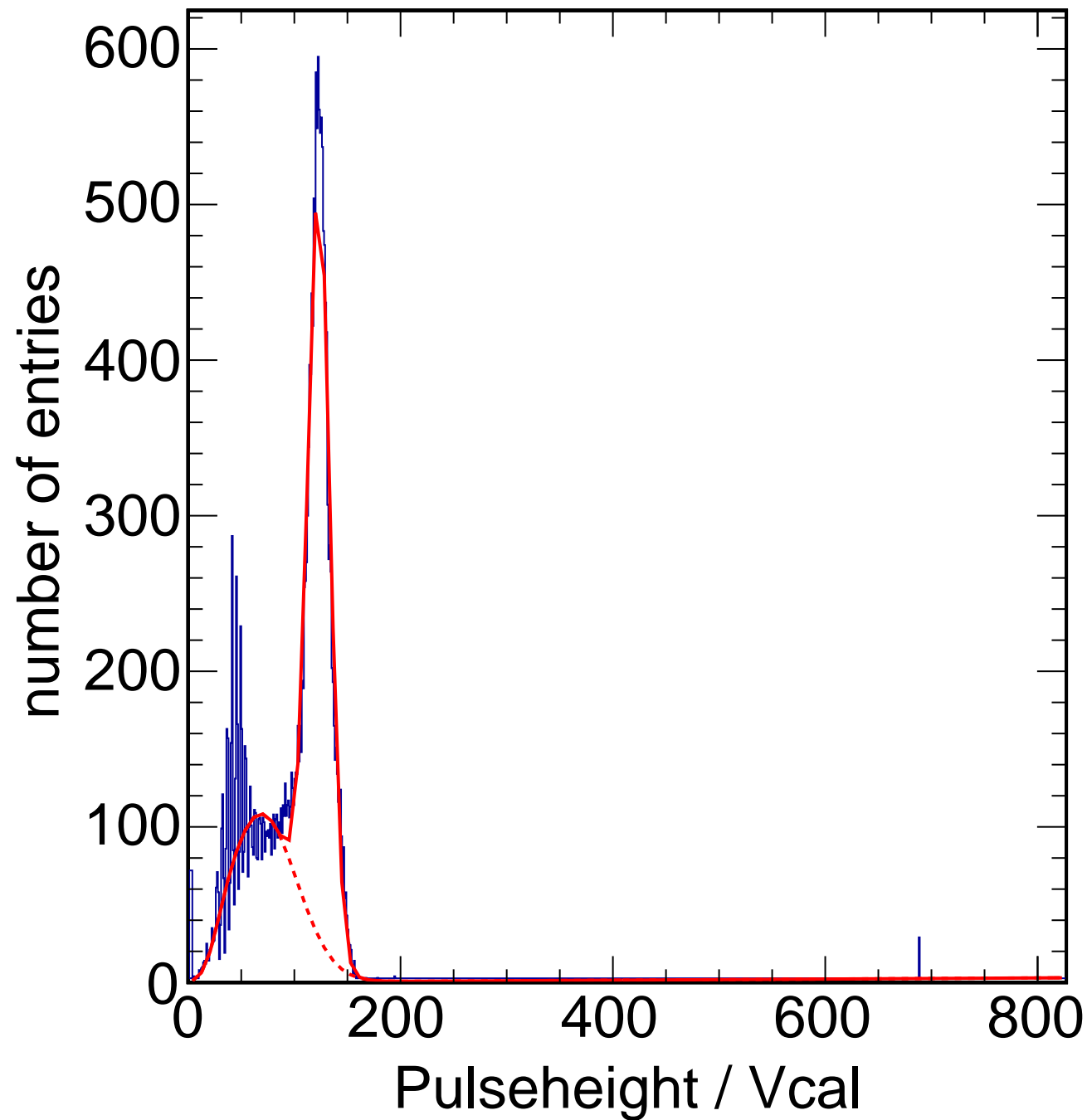
X-ray Calibration - Target Ag Method Spectrum Chip C12
