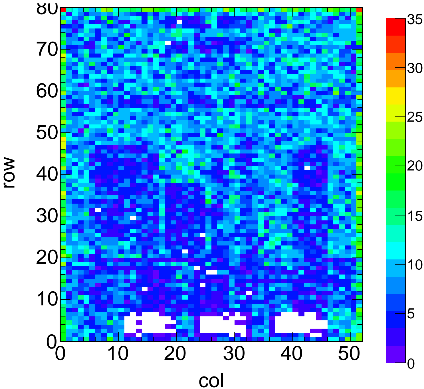
X-ray Hit Map - Target Zn Method Spectrum Chip C10
