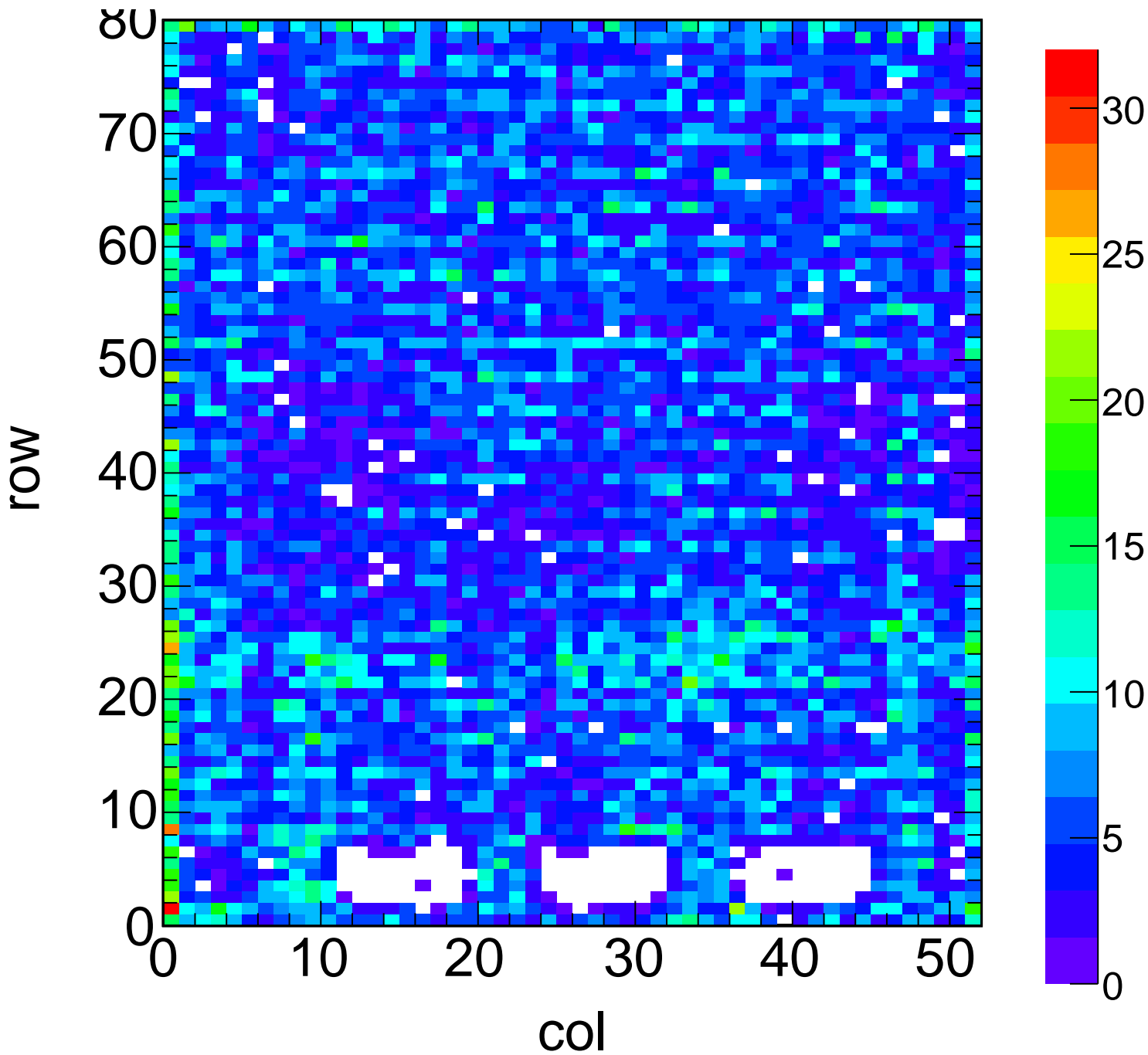
X-ray Hit Map - Target Zn Method Spectrum Chip C1
