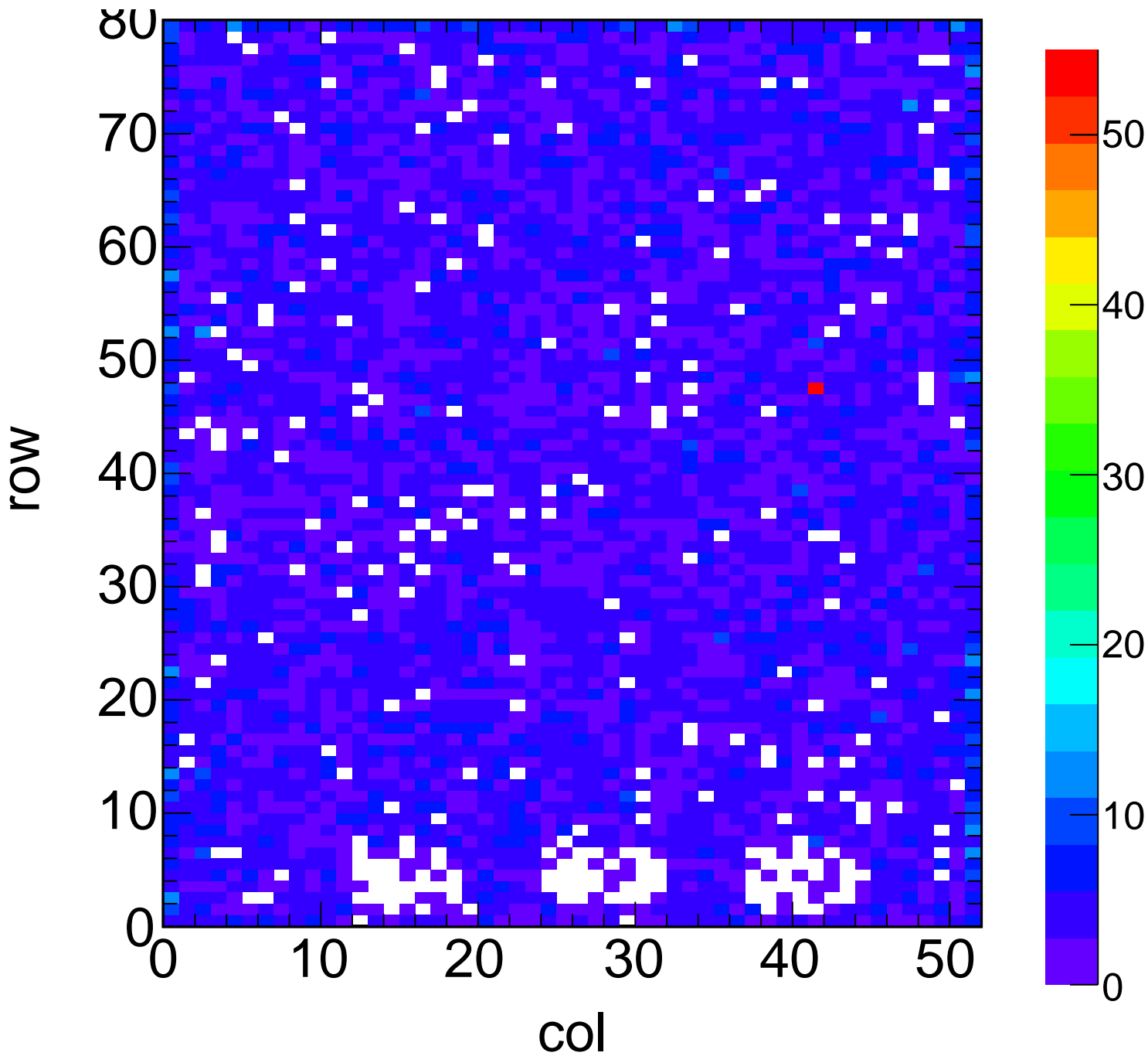
X-ray Hit Map - Target Sn Method Spectrum Chip C0
