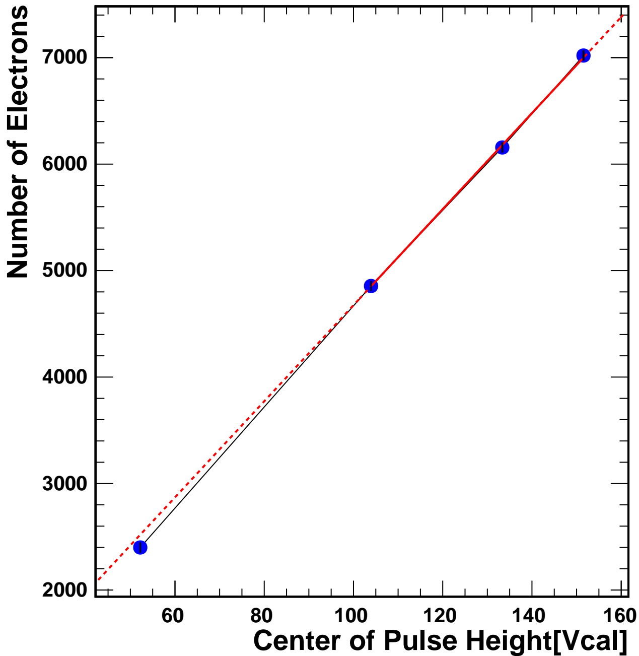
Center of Pulse Height (Vcal units) vs number of electrons
