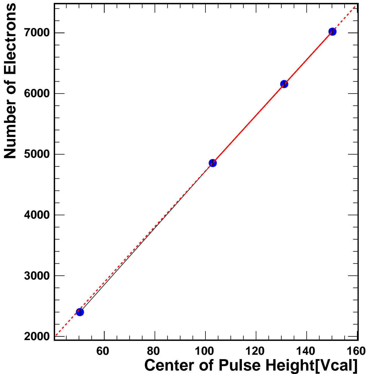
Center of Pulse Height (Vcal units) vs number of electrons
