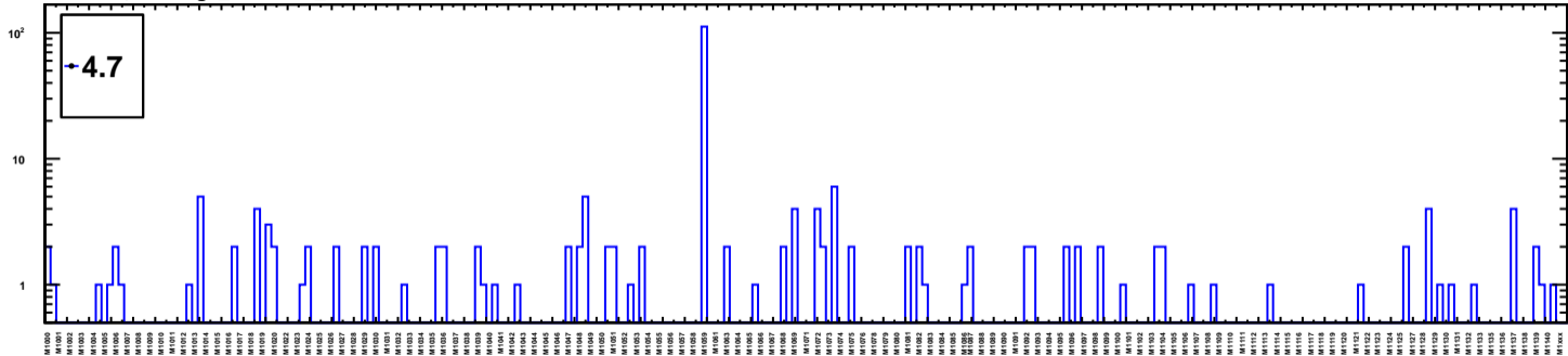
Fulltests, message_readback_count
