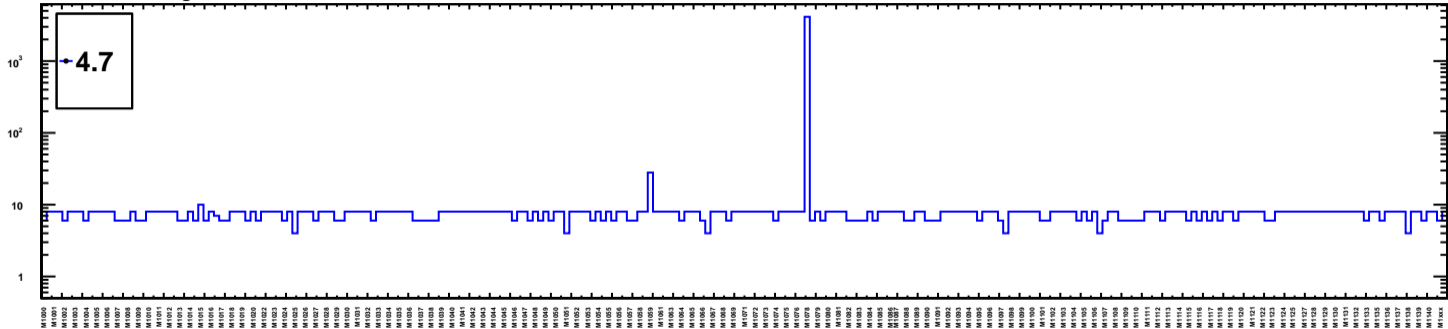
Fulltests, message_eventid_count
