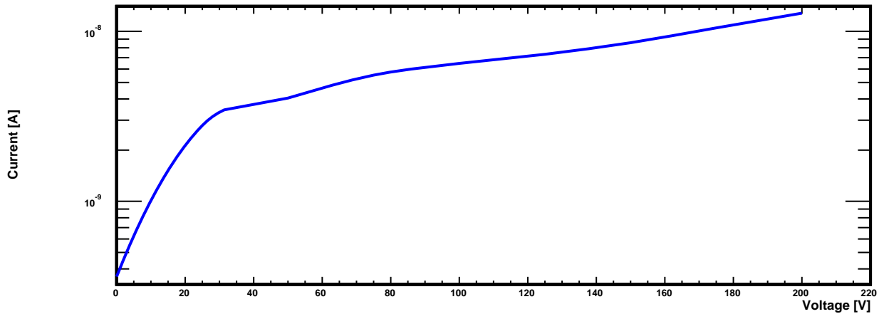
I-V-Curve
