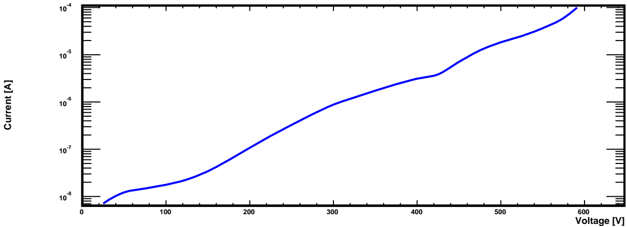
I-V-Curve
