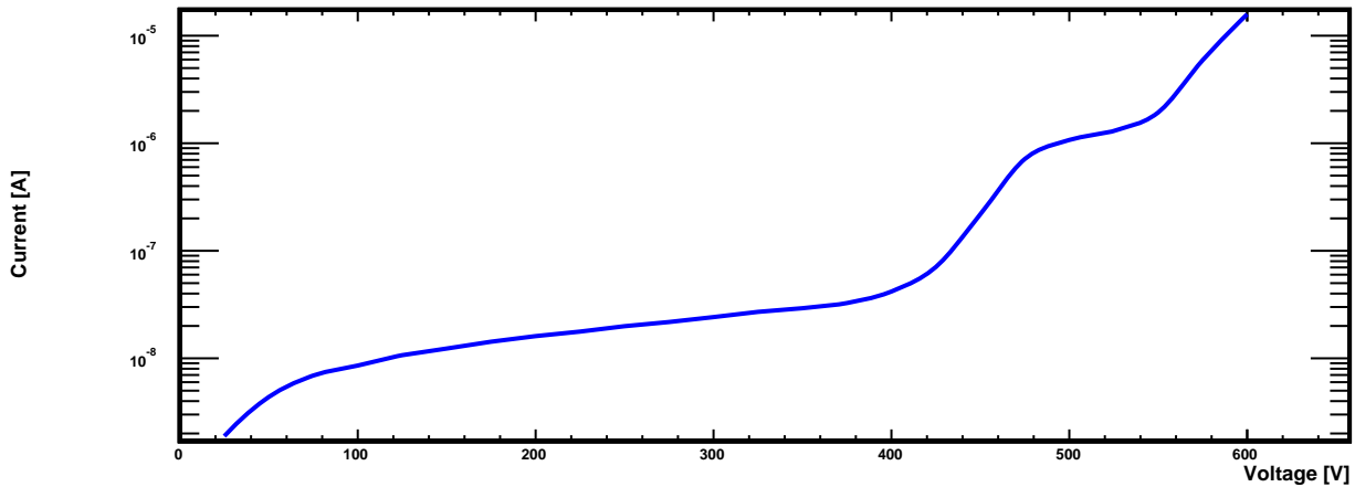
I-V-Curve
