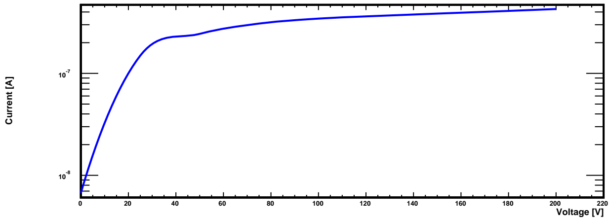
I-V-Curve
