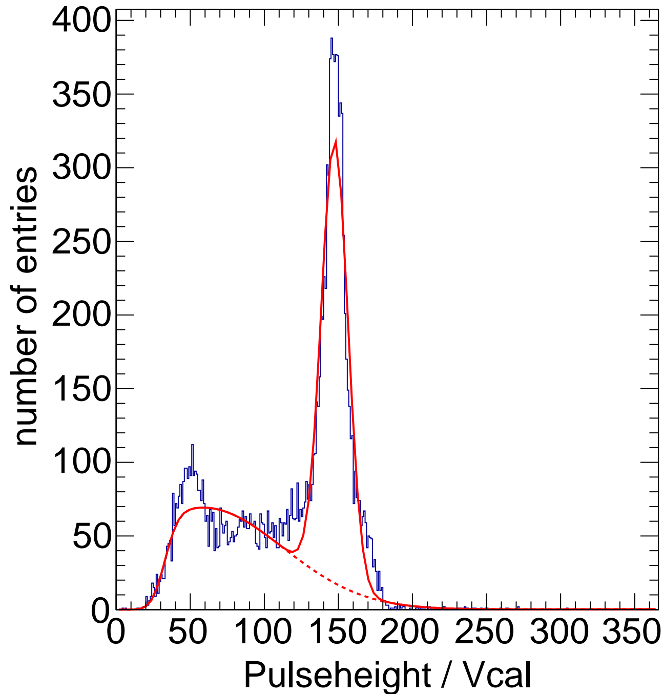
X-ray Calibration - Target Sn Method Spectrum Chip C11
