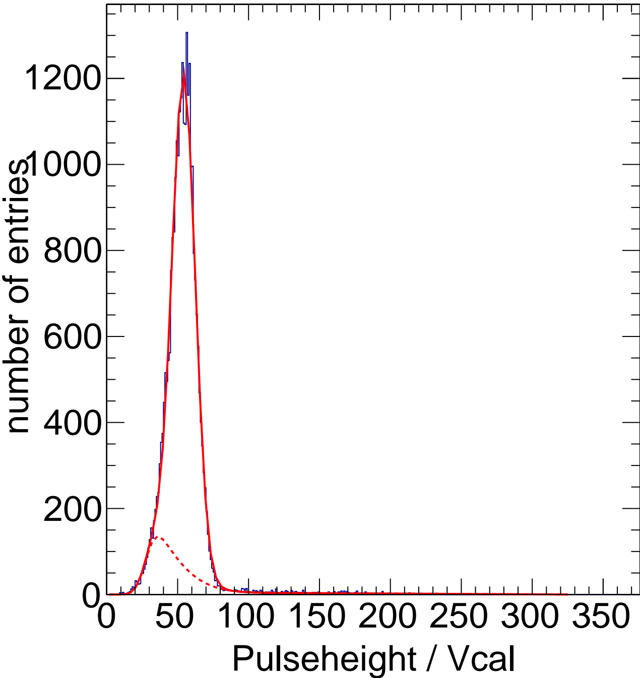
X-ray Calibration - Target Zn Method Spectrum Chip C7
