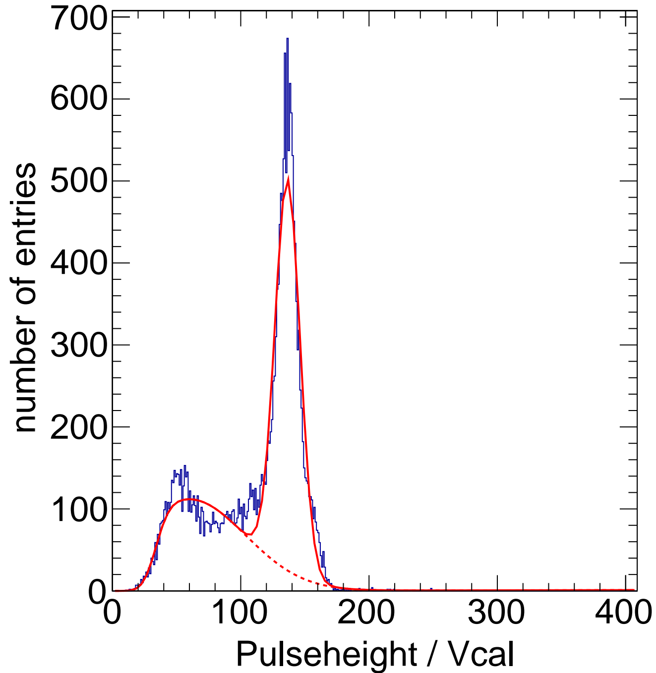
X-ray Calibration - Target Ag Method Spectrum Chip C7
