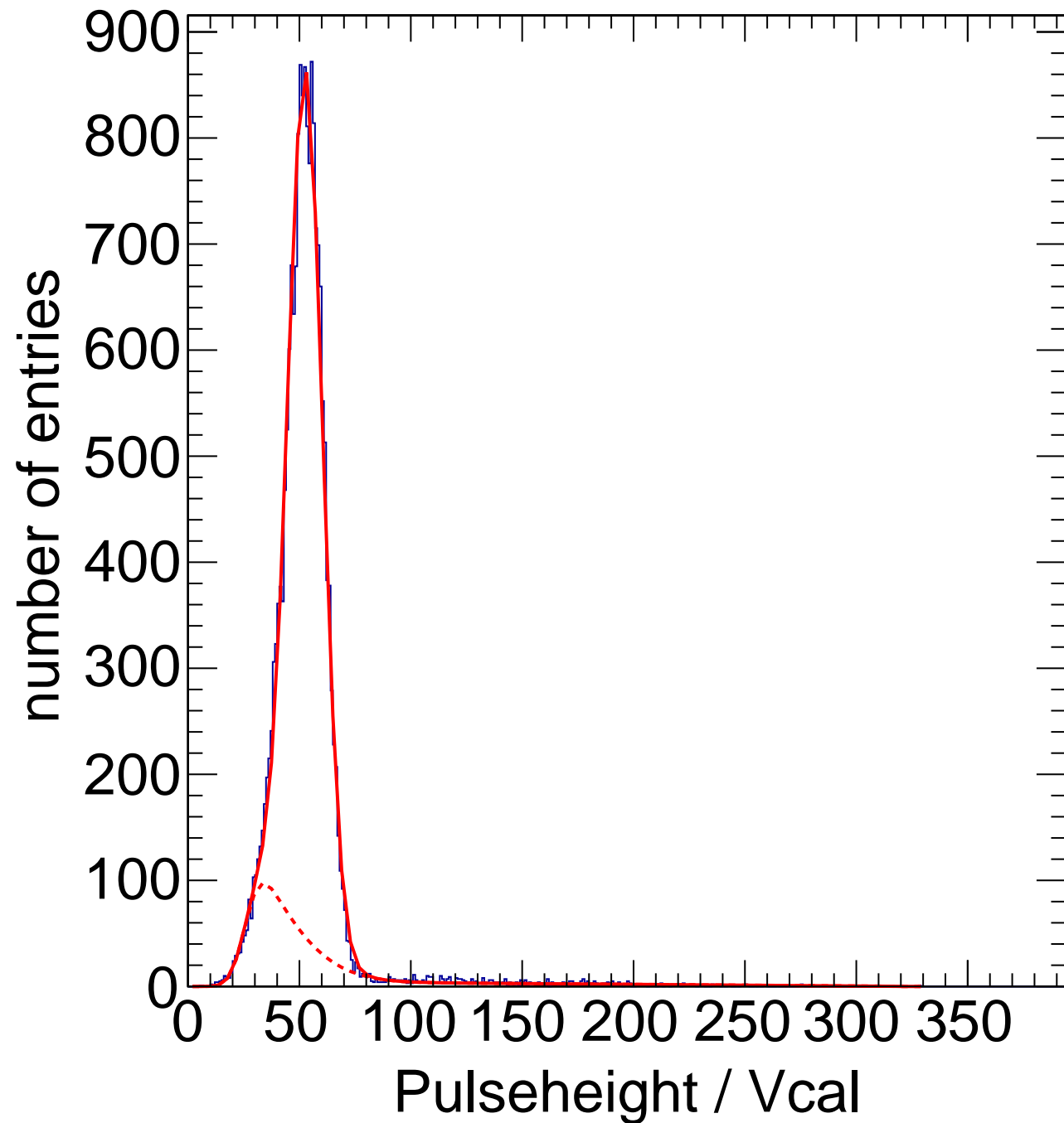
X-ray Calibration - Target Zn Method Spectrum Chip C14
