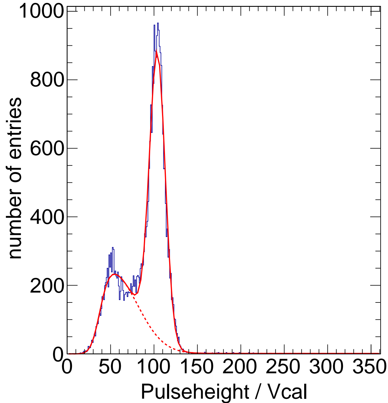
X-ray Calibration - Target Mo Method Spectrum Chip C1
