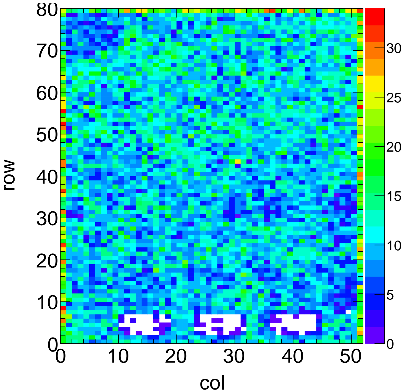
X-ray Hit Map - Target Mo Method Spectrum Chip C7
