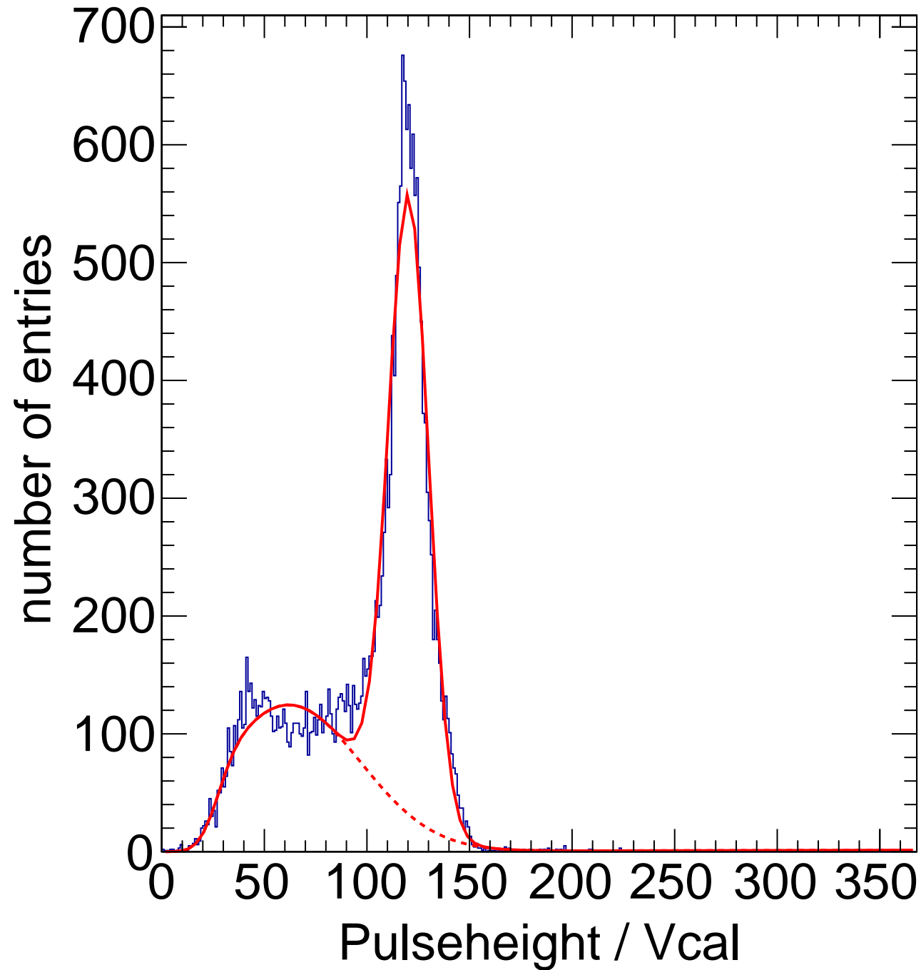
X-ray Calibration - Target Ag Method Spectrum Chip C3
