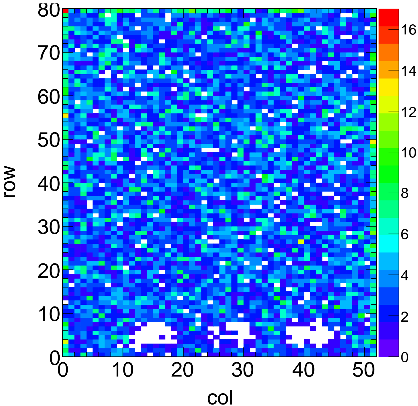
X-ray Hit Map - Target Sn Method Spectrum Chip C8
