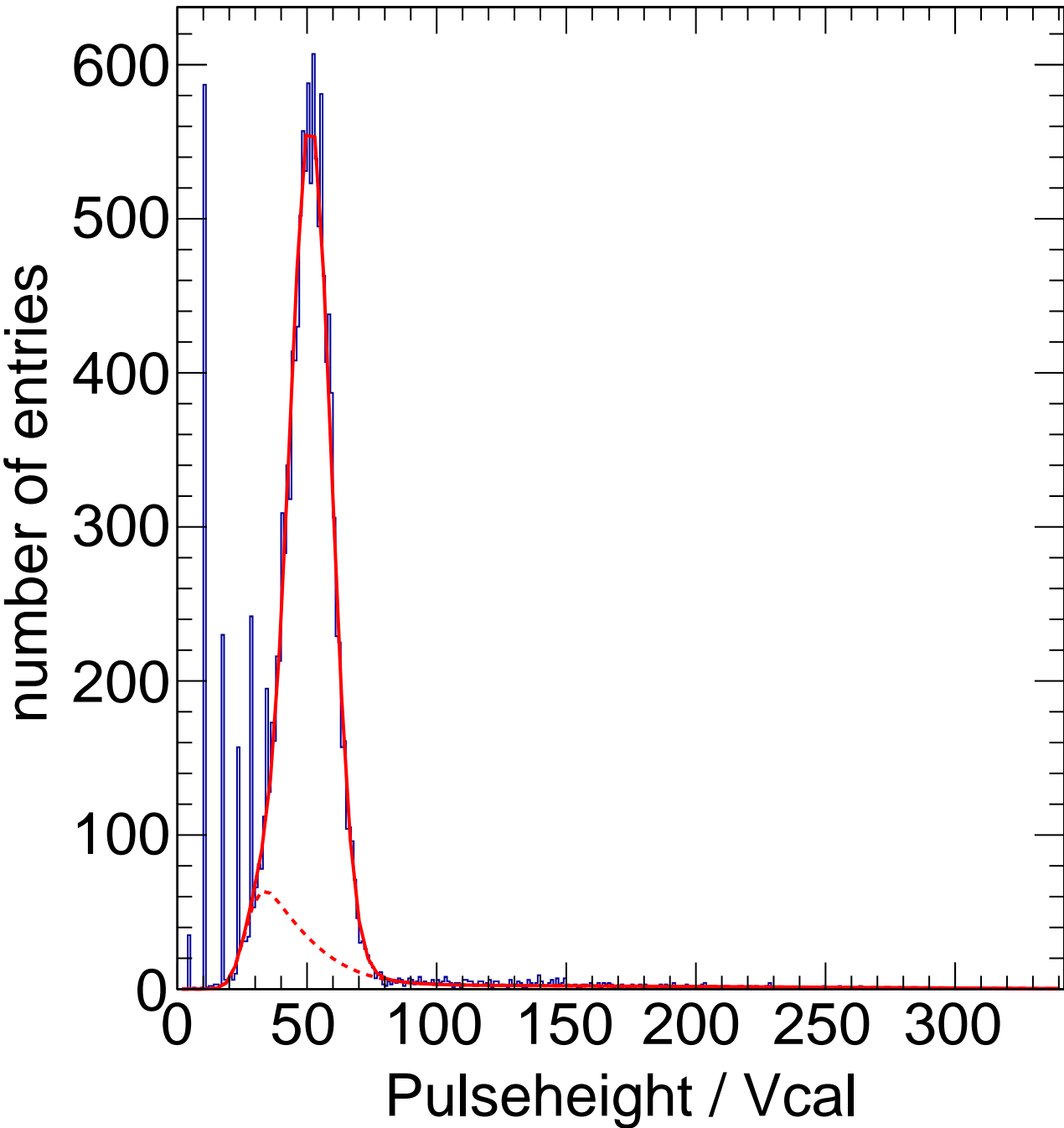
X-ray Calibration - Target Zn Method Spectrum Chip C2
