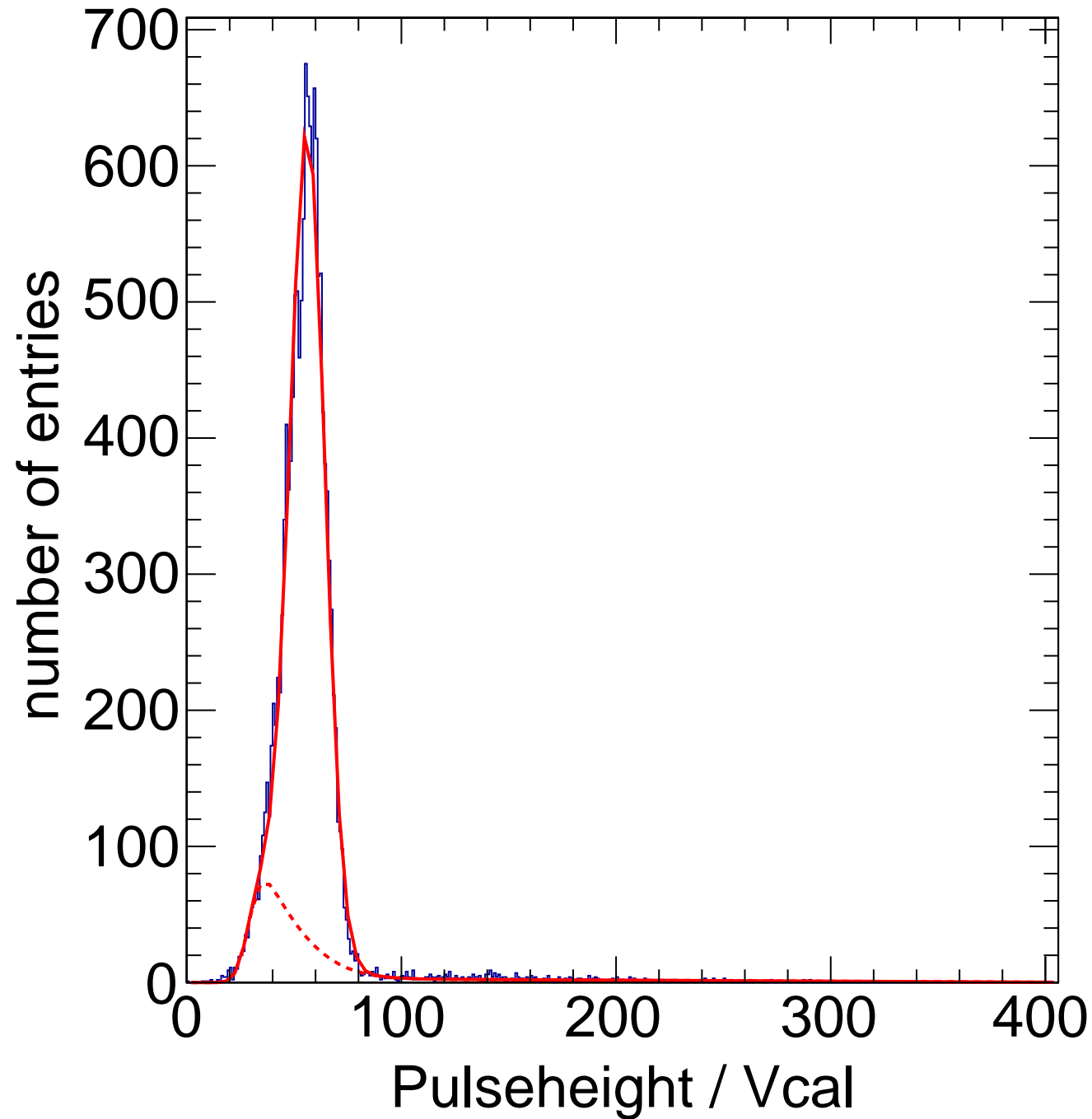
X-ray Calibration - Target Zn Method Spectrum Chip C13
