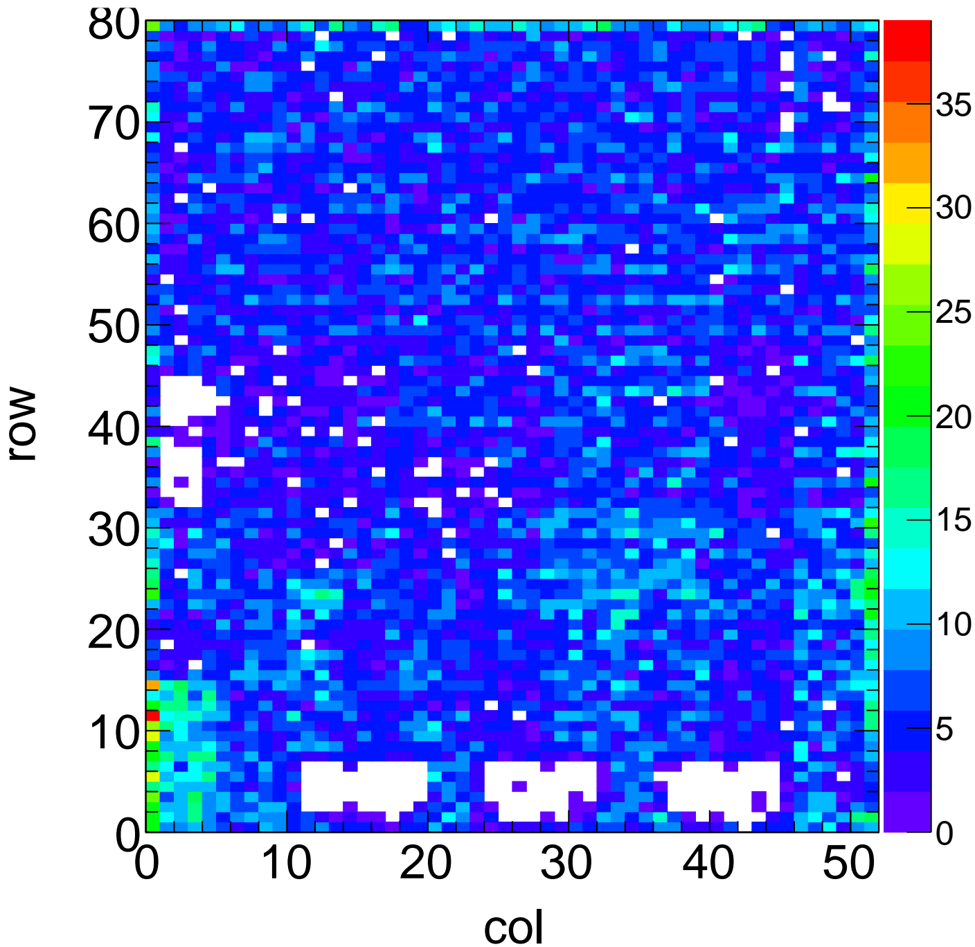
X-ray Hit Map - Target Zn Method Spectrum Chip C0
